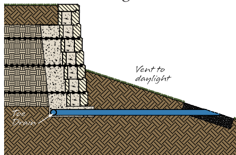
Vent to a lower grade
