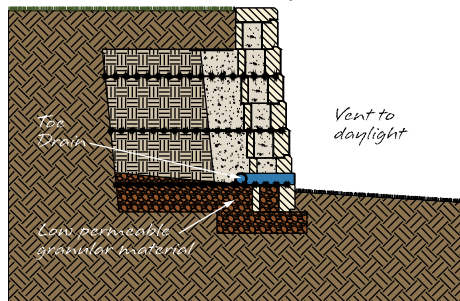
Vent thru the block face
