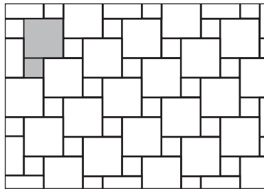
Double Half Pinwheel 80% 6x12 and 20% 6x6 or 80% 4.5x9 and 20% 4.5x4.5
